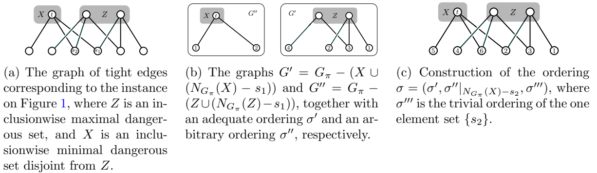
Figure 3: An illustration of the inductive step in Subcase 2.2.2.
