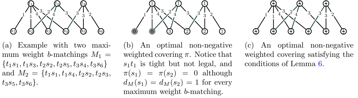
Figure 1: A bipartite graph corresponding to a market with three buyers having demand two and six items. The numbers denote the weights of the edges; missing edges have weight 0. There are two maximum weight b -matchings M_1 and M_2 . Note that both s_3t_1 and s_4t_1 are legal, but they do not form a feasible set.
