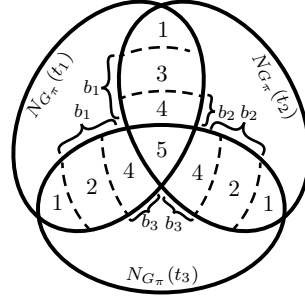
Figure 2: Definition of the labeling \Theta for three buyers. Some parts might be empty, e.g. if |X_{12}| \leq b_2 , then there are no items with label 1 and 3 in the intersection of N_{G_\pi}(t_1) and N_{G_\pi}(t_2) .
