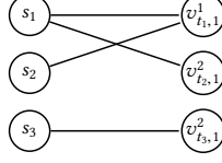
Fig. 5. school priority s_1 \succ_c s_2 \succ_c s_3
