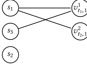
Fig. 6. school priority s_1 \succ_c s_2 \succ_c s_3
