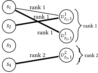
Fig. 3. The maximal diversity matching for ranked reservation graph of school c_1 in Example 2.1 is illustrated by thick bold edges.
