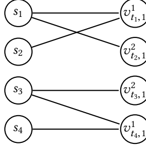
Fig. 4. The corresponding reservation graph of school c in Example 6.4.
