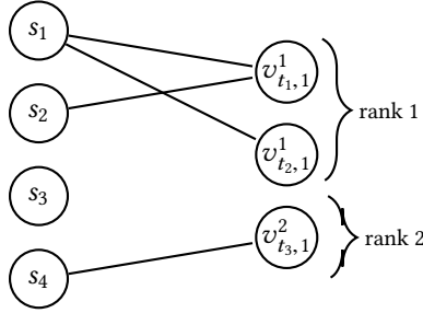
Fig. 2. The ranked reservation graph of school c_1 in Example 2.1.
