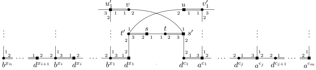
Fig. 3. Illustration of the reduction in the proof of Theorem 5, depicting the part of graph \hat{G} where it differs from graph \tilde{G} (shown in Figure 2). Double lines denote the matching \tilde{M}_0 .
