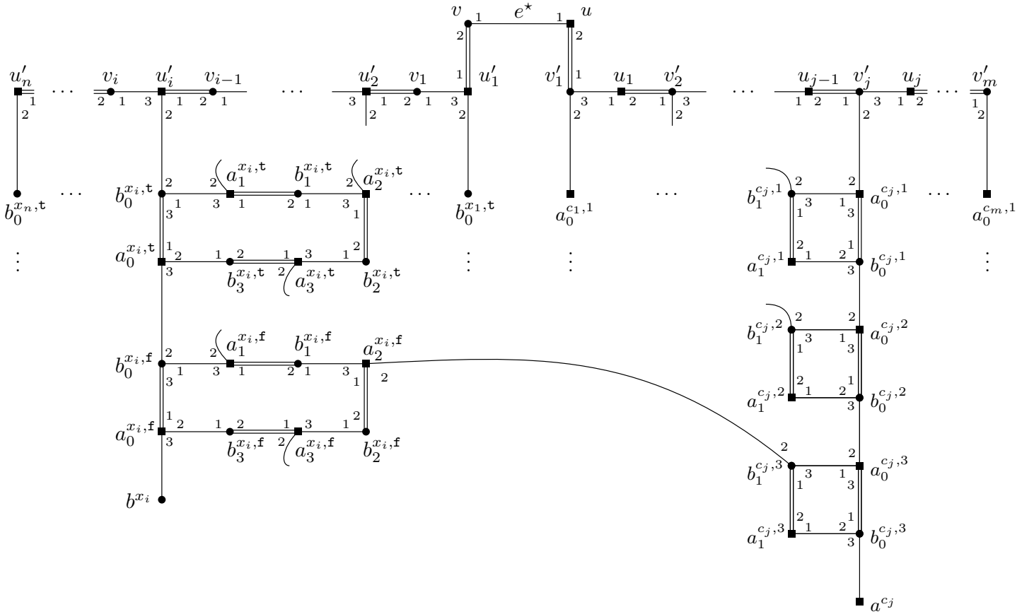
Fig. 2. Illustration of the reduction in the proof of Theorem 3. Edges of \tilde{M}_0 are depicted as double lines. The figure only shows one consistency edge, corresponding to a situation where the third literal in c_j is x_i as a positive literal.
