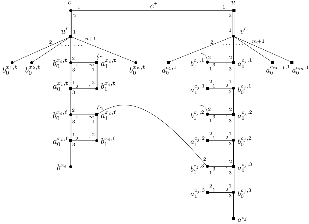
Fig. 1. Illustration of the reduction in the proof of Theorem 15. Edges of M_0 are depicted as double lines. The figure only shows one consistency edge, corresponding to a situation where the third literal in c_j is x_i as a positive literal.
