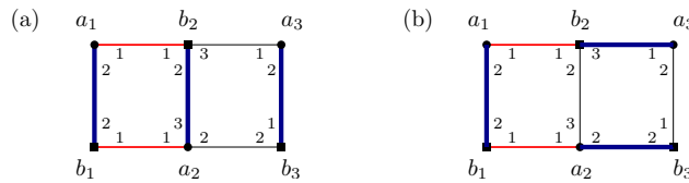
Fig. 7. An example illustrating why the simplest approach for finding a Pareto-optimal matching with at most k blocking edges and maximal utility does not work.
