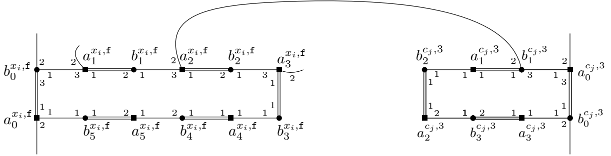
Fig. 5. Illustration of the reduction in the proof of Theorem 11, depicting how the graph \tilde{G} is modified to obtain graph \tilde{G}^{\text{ties}} . The figure assumes that the third literal in c_j is x_i as a positive literal. Edges leaving a given vertex a that are labelled with the same rank lead to vertices that are equally preferred by a and hence are contained in a tie in a 's preference list.
