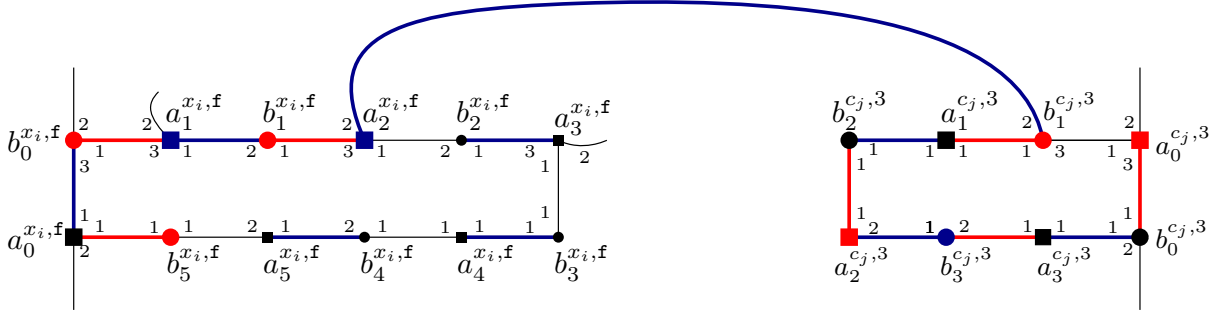
Fig. 6. Illustration of the matching M' in the proof of Theorem 11 in the case where the matching M (depicted in blue) contains the consistency edge (a_2^{x_i, \mathbf{f}}, b_1^{c_j, 3}) . The figure assumes (a_0^{x_i, \mathbf{f}}, b_0^{x_i, \mathbf{f}}) \in M but (a_0^{c_j, 3}, b_0^{c_j, 3}) \notin M . Edges of M' \setminus M are depicted in red. Vertices in V(M \triangle M') are emphasized by their somewhat greater size. Furthermore, vertices that prefer M' to M are shown in red, while those preferring M to M' are blue; indifferent vertices are black.
