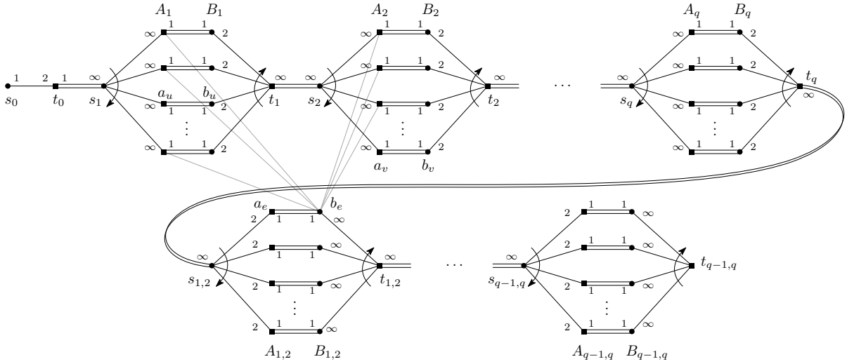
Fig. 4. Illustration of the reduction in the proof of Theorem 9. Vertex gadgets are shown in the upper row, with edge gadgets below them. We assume \mu(i) = i for each i \in [q] , as well as \mu(q+1) = (1, 2) and \mu(q + \binom{q}{2}) = (q-1, q) . Double lines denote edges of M_s . Among consistency edges only those incident to b_e are shown, in grey. The figure assumes e = (u, v) \in E_{1,2} .
