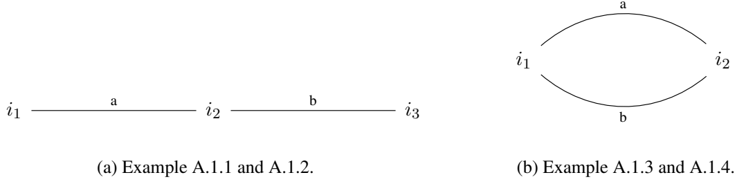
Figure 7: Contracts in Example A.1.
