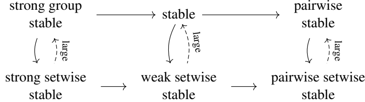
Figure 5: Summary of the relationships between stability concepts. The regular arrows represent obvious relationships between stability concepts, the dashed arrows relationships that rely on markets being large.
