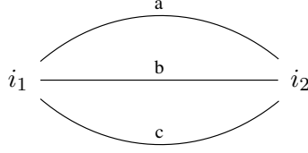
Figure 6: Contracts in Example 1.
