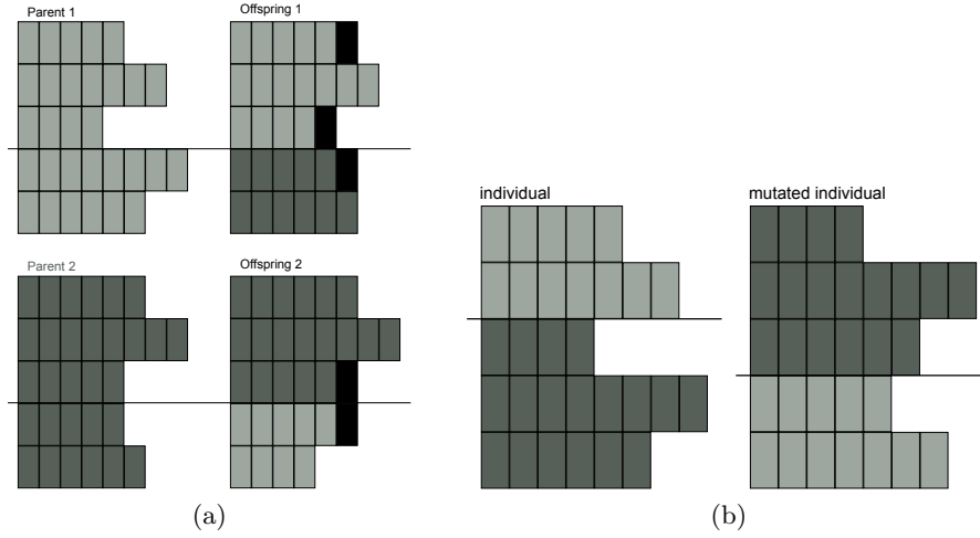
Fig. 1: Schematic representations of (a) the horizontal block crossover and (b) the horizontal flop mutation.
