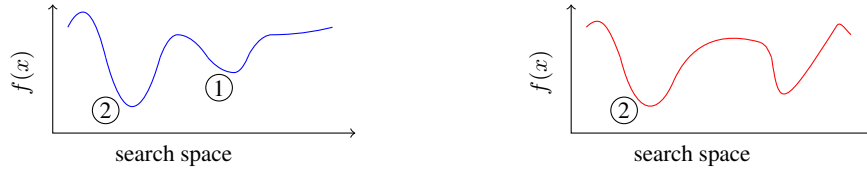
Figure 3.1: objective functions for neighborhoods A and B
