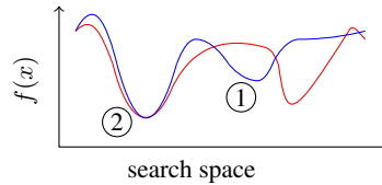
Figure 3.2: combined objective function for neighborhoods A and B
