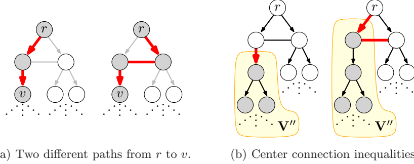
Fig. 2. Triangle tree: In the odd diameter case there are two paths connecting r with any node v \in V . This leads to the center connection inequalities involving the center edge.
