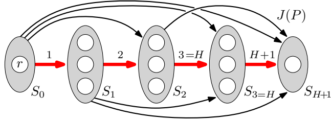
Fig. 1. Partitioning P of the nodes in V^+ into H + 2 nonempty sets S_0, \dots, S_{H+1} . The jump J(P) contains all arcs leading from a partition to a higher indexed one skipping at least one in-between (curved arcs). A path connecting r with nodes in S_{H+1} without any arc from J(P) would consist of at least H + 1 arcs and thus violate the hop constraint H .
