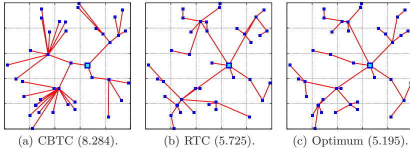
Fig. 5. Diameter constrained trees computed by two different construction heuristics, CBTC and RTC (best solution from 100 runs), and the optimal solution (complete, Euclidean graph with 40 nodes distributed randomly in the unit square, D = 6 ). Corresponding objective values are given in parenthesis. Heuristics were forced to use the center of the optimum.
