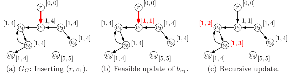
Fig. 4. Insertion of arc (r, v_1) into the constraint graph G_C , including all necessary updates to the assignment intervals.
