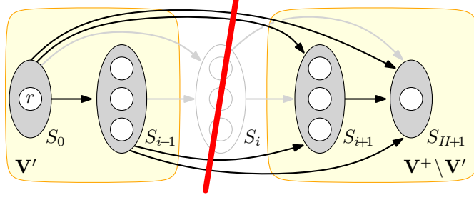
Fig. 3. A partitioning P with \sum_{J(P)} x^{\text{LP}} < 1 and an empty set S_i corresponds to a violated directed connection cut.
