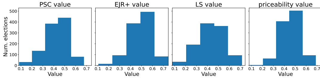
Figure 1: Histograms of optimal \alpha -values achievable in our elections, rounded to one decimal place.
