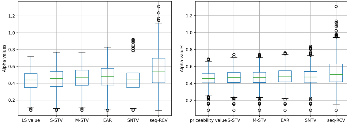
Figure 4: The LS and priceability values achieved by voting rules
