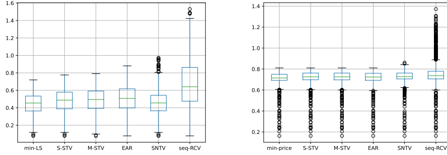
Figure 7: The LS and priceability values achieved by voting rules (completed preferences).
