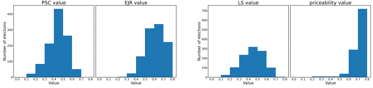
Figure 5: Histograms of optimal values, rounded to one decimal place (completed preferences).
