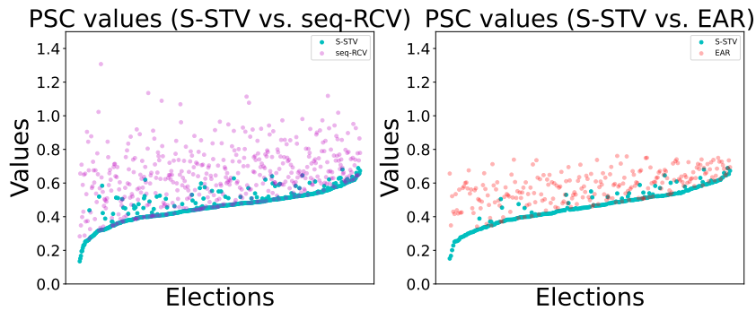
Figure 3: Left: PSC values achieved by Scottish STV and seq-RCV for the 485 elections where the rules disagree. Right: PSC values achieved by Scottish STV and EAR over the 262 elections where the rules disagree. Elections are ordered by increasing optimal PSC value.
