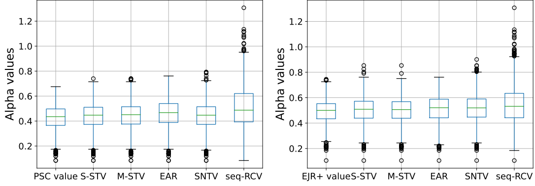
Figure 2: Left: The PSC values achieved by voting rules, together with optimal PSC values (shown in the leftmost column). Right: The EJR+ values achieved by voting rules, together with optimal EJR+ values (shown in the leftmost column).
