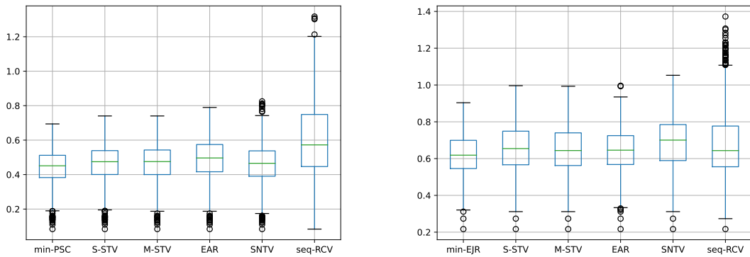
Figure 6: The PSC and EJR+ values achieved by voting rules (completed preferences).
