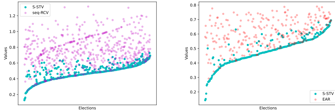
Figure 8: Left: Differences in PSC values between Scottish STV and Sequential RCV when elections where the rules agree are excluded (completed preferences). Right: Differences in PSC values between Scottish STV and EAR when elections where the rules agree are excluded (completed preferences). Elections are ordered by increasing optimal PSC value.
