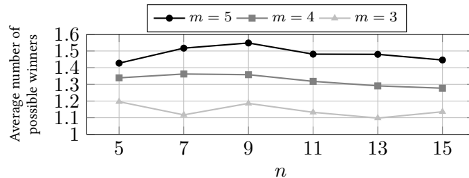
Figure 1: Average number of possible iterative winners in function of n (for m \in \{3, 4, 5\} )
