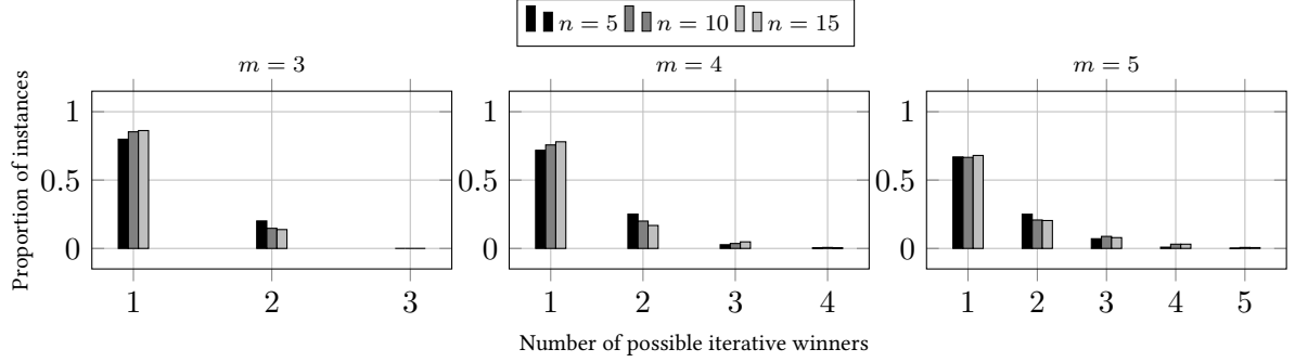
Figure 2: Distribution of the number of possible iterative winners in function of n (for m \in \{3, 4, 5\} )
